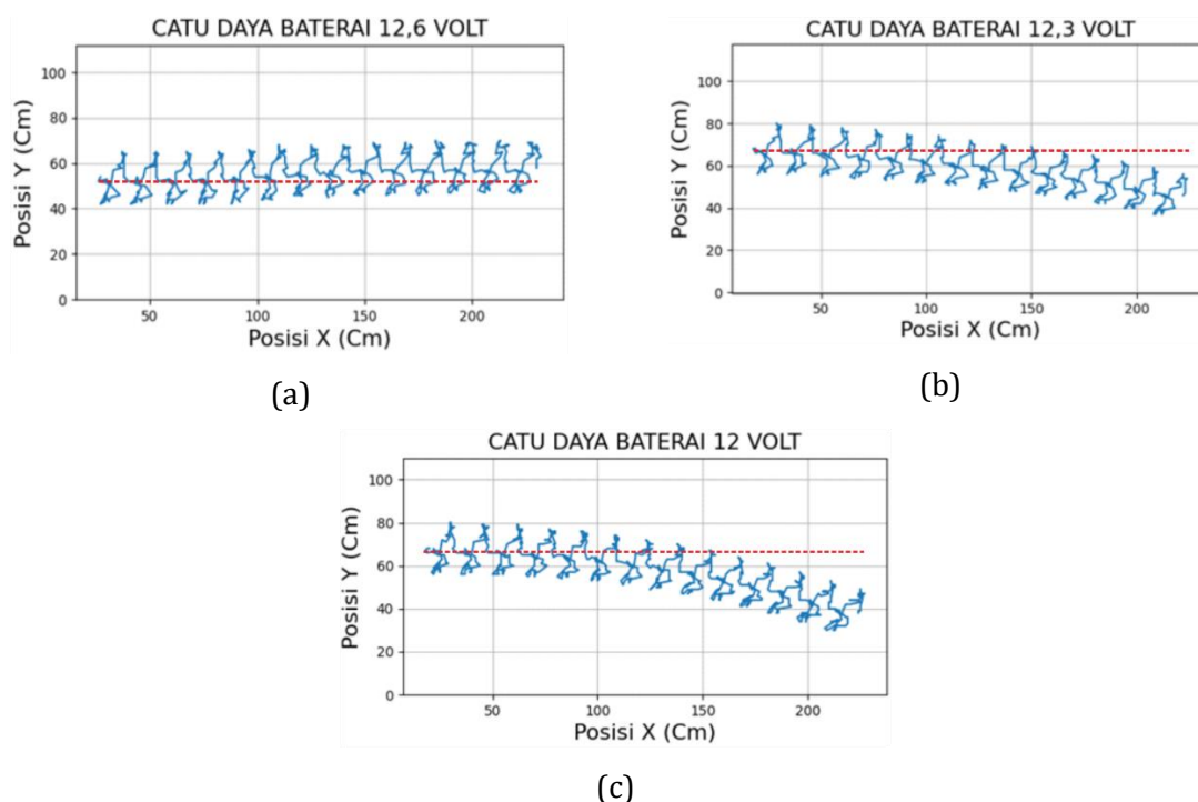
Figure 10. Battery Power Supply 12.6V, (b) Battery Power Supply 12.3V (c) Battery Power Supply 12V
