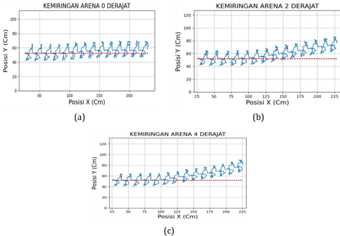
Figure 11. (a) Arena slope 0^\circ , (b) Arena slope 2^\circ , (c) Arena slope 4^\circ
