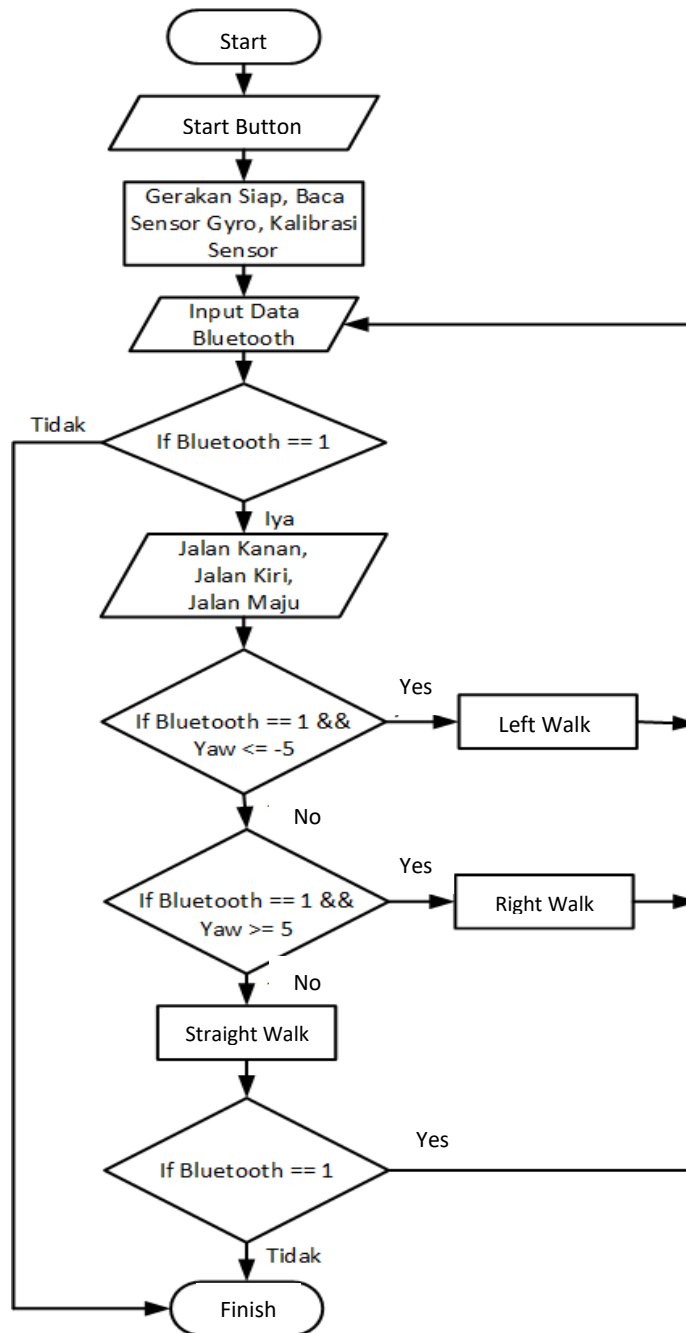
Figure 6. Flowchart
