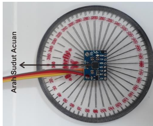
Figure 8. Testing the sensor against the protractor angle
