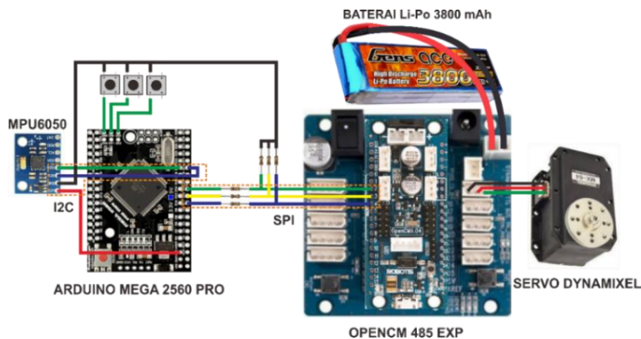
Figure 5. Wiring Diagram
