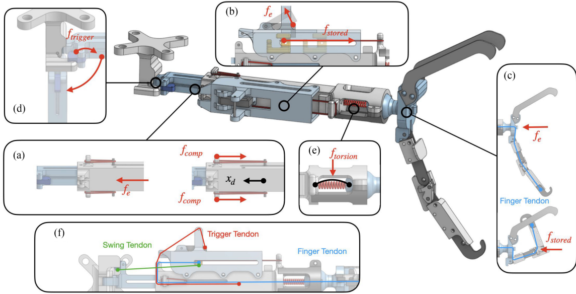
Fig. 4. Detailed gripper mechanism. (a) shows the main linear compliance mechanism consists of two segments of the main gripper body and rubber bands. (b) shows the gripper trigger mechanism where upon impact force releasing the trigger, the stored energy is used to close the gripper and hold the position. (c) shows the underactuated finger where upon impact force releasing the trigger, the stored energy is used to close the gripper and hold the position. (d) shows the optional swinging mechanism that enables the gripper to swing down after impact. (e) shows the ball joint connecting the under-actuated finger to the main body of the gripper, with a compression spring embedded in the structure to provide the rotational compliance, and (f) illustrates the three tendons used in the gripper mechanism and its routing.
