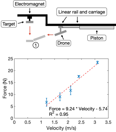
Fig. 7. Top: illustration of linear rail setup. The grasping drone is mounted on a linear rail. A piston accelerates the carriage drone to the desired exit velocity. A target drone is released through the control of an electromagnet. The timing is set such that the drone and target collide at point (1) while both are in ballistic motion. Bottom: the relationship between relative velocity and the measured peak impulse force at collision. The range of flight data collected at each velocity is marked with error bars with an average. A linear fit relates the velocity and peak impact force.
