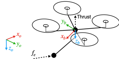
Fig. 2. Quadrotor schematic.
