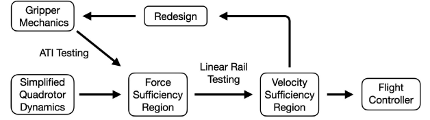
Fig. 3. Road-map to employ the velocity sufficiency region.
